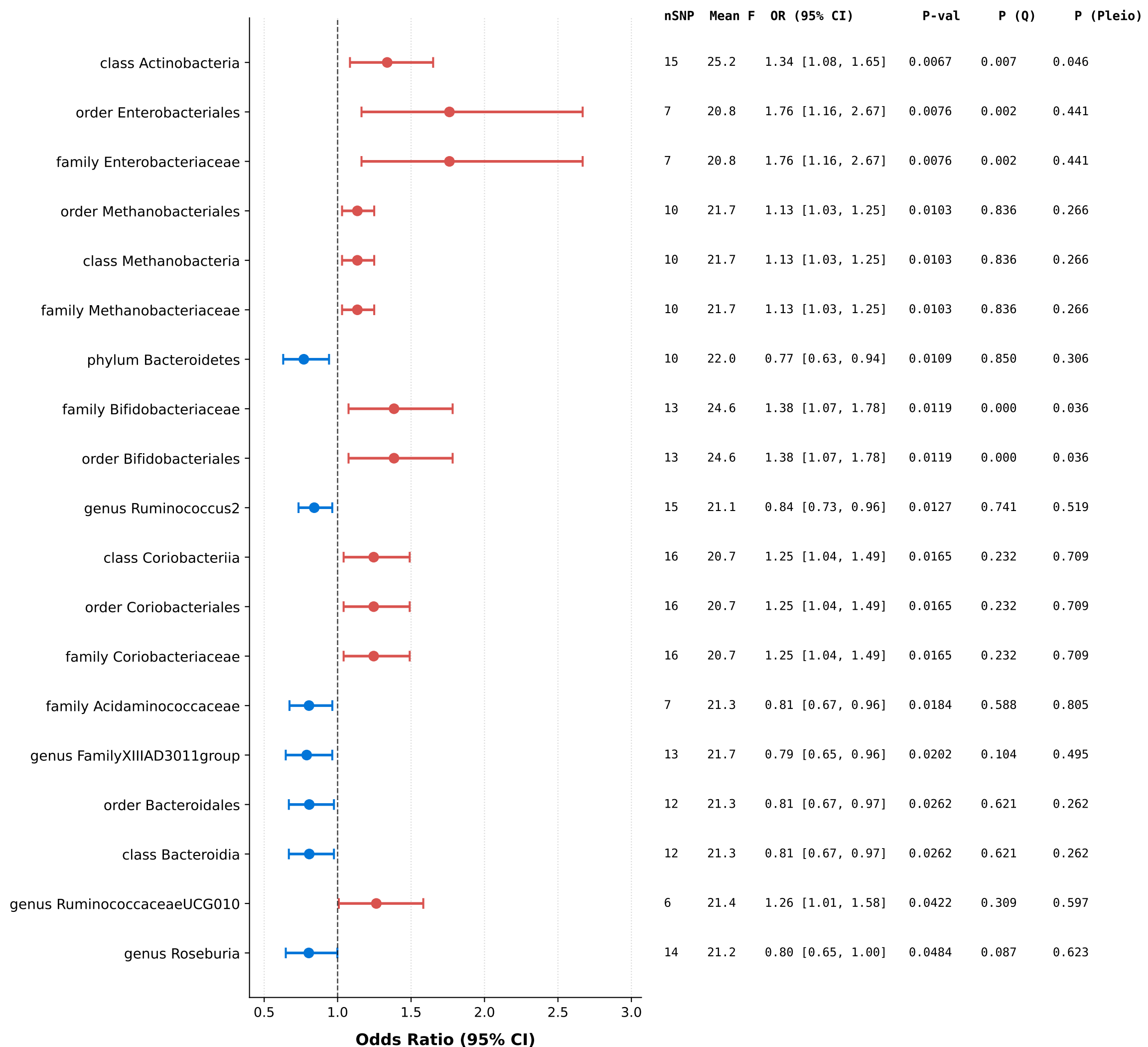
Forest Plot: Colorectal Adenocarcinoma (with Complete Test Statistics)
